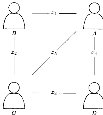
Figure 2: Visualization of a dining cryptographers network. Participant A shares the coin flip outcome x_1 with participant B , x_4 with D and x_5 with C . Note that participant B and D do not share a coin flip outcome.
